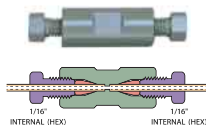
Internal union – PEEK Standard bore version (ZU1PK)
