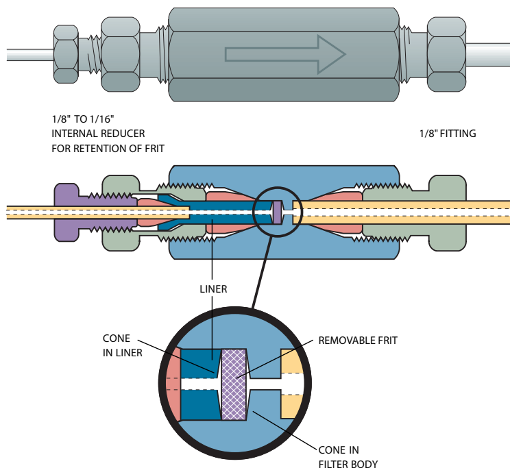
Reducing filter with a removable frit 1/8" to 1/16" (ZRUFR21F)
