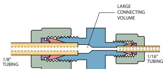
Figure 7: Common commercial reducing union
