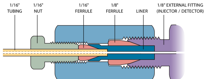
External to internal reducer (EZR21)
