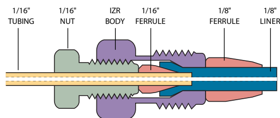
Valco's unique internal reducer (IZR21)
