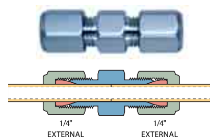
External union
