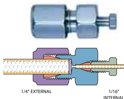
Analytical external column end fitting with removable frit (ECEF414.6F)
