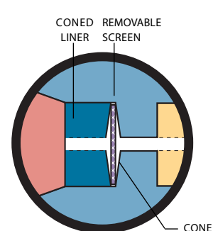
Removable screen
