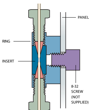
Panel mounting
