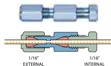
External/internal union
